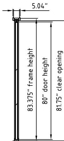
Cross section B - B
