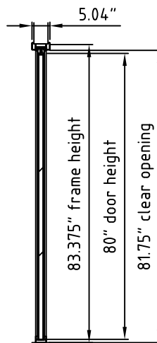
Cross section B - B
