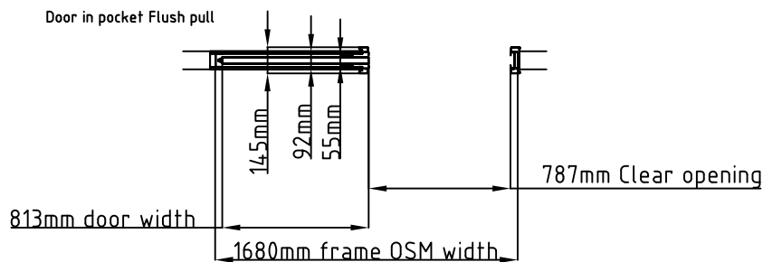
Door in pocket Flush pull
